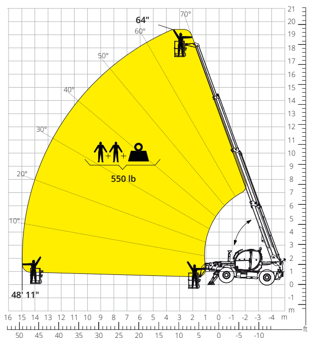
Load chart with FIXED PLATFORM, 550 lb AT-01-001
